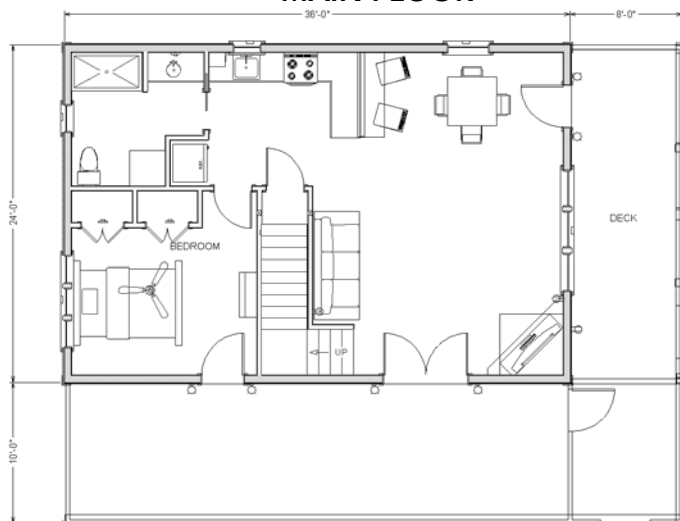
MAIN FLOOR
