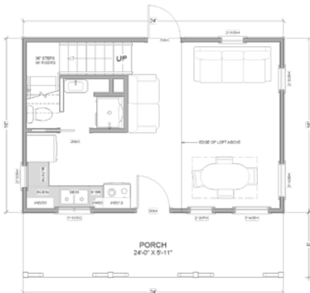
Main Floor
