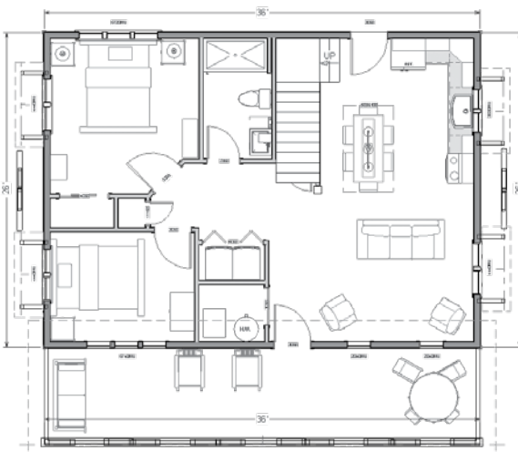
MAIN FLOOR
